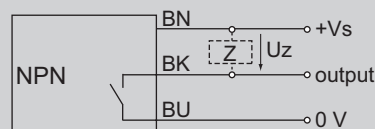
NPN normally open (NO)
