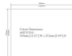
Panel Cutout
