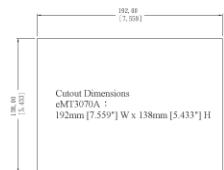
Panel Cutout
